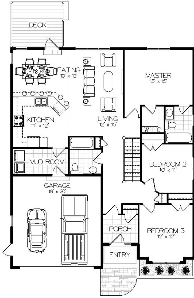
MAIN FLOOR
