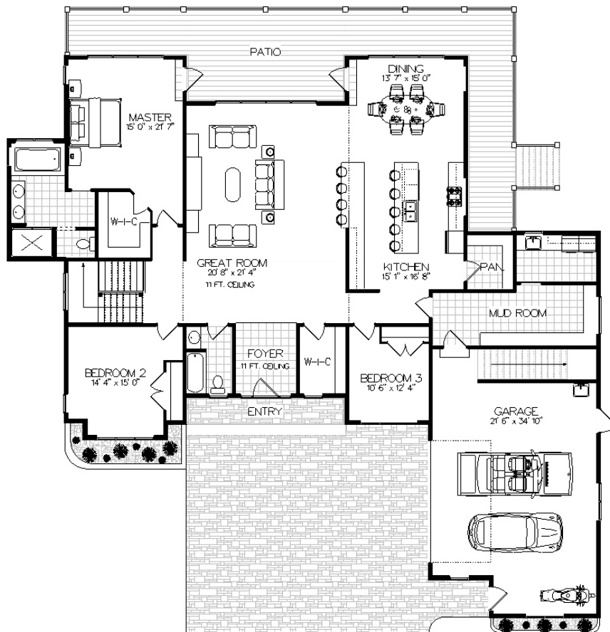
MAIN FLOOR
